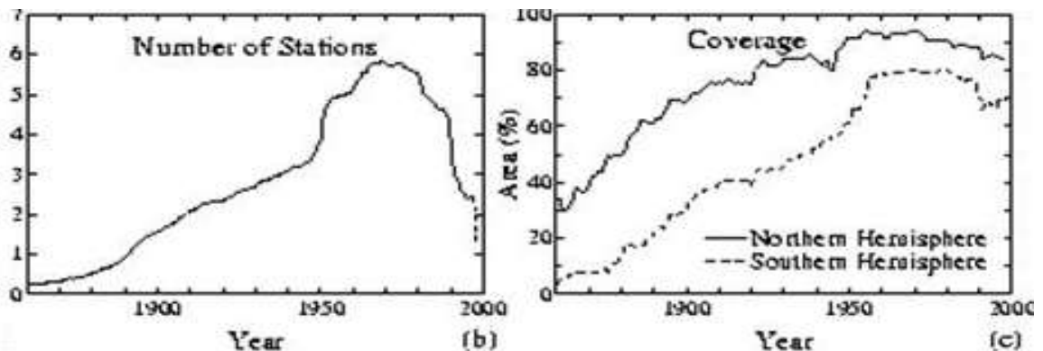
Figure 4.12: Number of weather stations and global coverage (%) over time.
