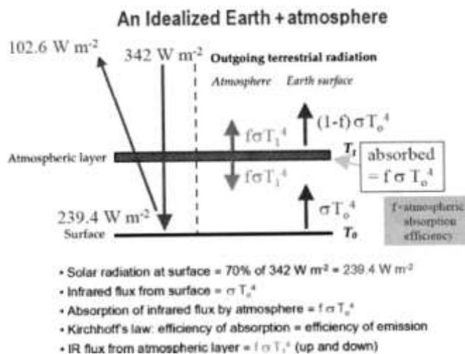
Figure 2.4: A simplistic greenhouse model of radiation at Earth's surface and atmospheric layer
