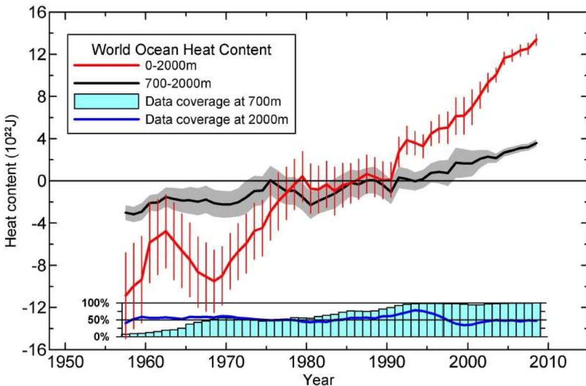
Figure 4.4: World ocean heat content ( 10^{22} J) for the 0-2000m (red) and 700-2000m (black) layers based on running pentadal (five-year) analyses. Reference period is 1955-2006. Each pentadal estimate is plotted at the midpoint of the 5-year period. The vertical bars represent \pm 2 times the standard error of the mean (S.E.) about the pentadal estimate for the 0-2000m estimates and the grey-shaded area represent \pm 2 *S.E. about the pentadal estimate for the 700-2000m estimates. The blue bar chart at the bottom represents the percentage of one-degree squares (globally) that have at least four pentadal one-degree square anomaly values used in their computation at 700m depth. Blue line is the same as for the bar chart but for 2000m depth. From Levitus et al. (2012) 38
