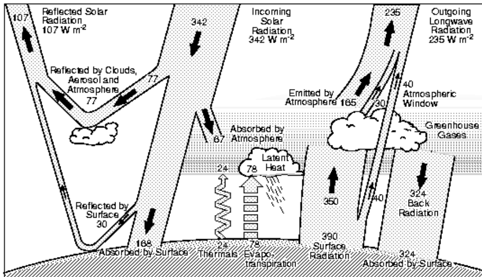
Figure 2.5: The Kiehl-Trenberth Energy Budget for Earth (1997)
