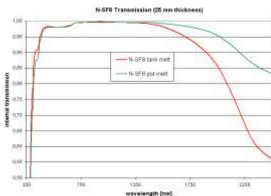
Figure 1.7: Comparison of typical transmittance curves of N-SF6 from two different melting techniques.
