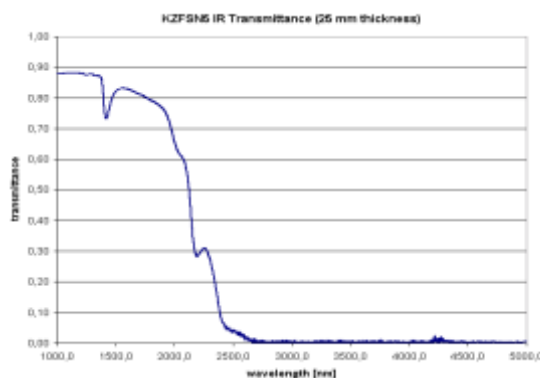
Figure 1.8: Infrared transmittance curve of KZFSN5 Source: SCHOTT AG
