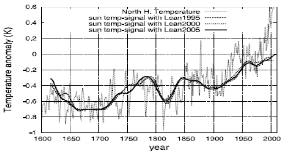
Figure 3.8: Parallel trends in solar irradiance and Northern Hemisphere temperatures.
