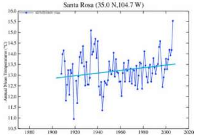
Figure 4.9: Processed GISS data showing warming
