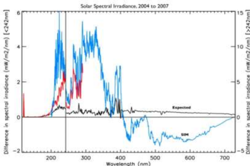
Figure 3.7: NASA's Solar Irradiance Monitor (SIM) measurements across the spectrum: 2004-2007.
