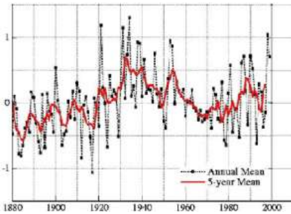
Figure 4.10: GISS 1999 processed US temperature data
