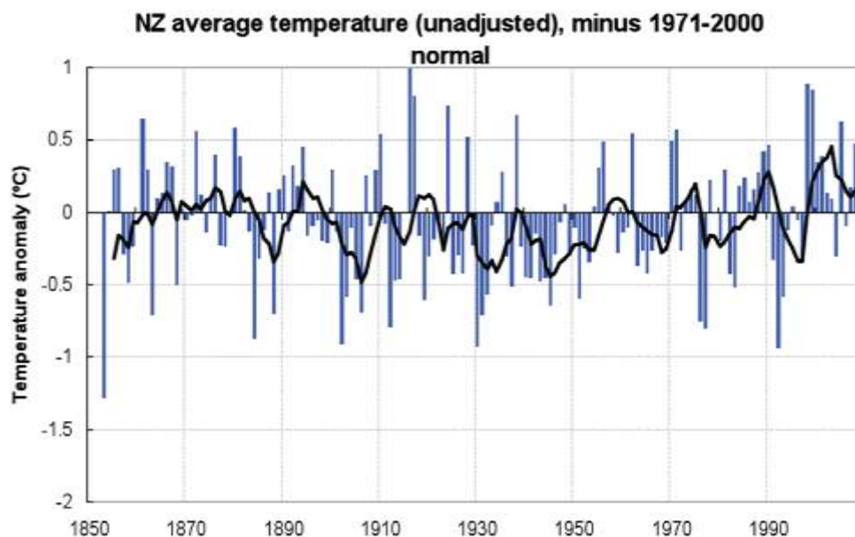
Figure 4.1: Temperature anomaly based on raw New Zealand temperature data (1850-2009)
