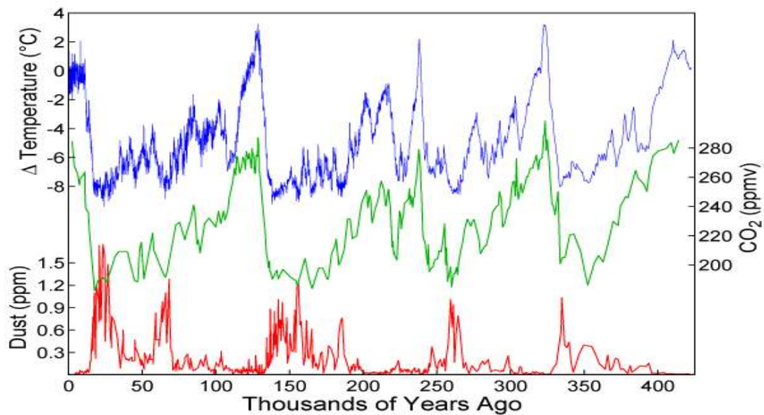
Figure 3.2: Temperature, CO 2 and dust record from the Vostok ice core over the past 420,000 years.
