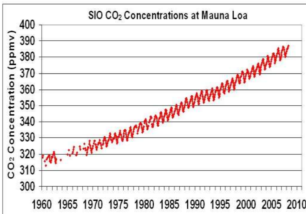
Figure 3.1: Atmospheric CO 2 levels at Hawaii's Mauna Loa Station, 1960-2009. Source: CDIAC
