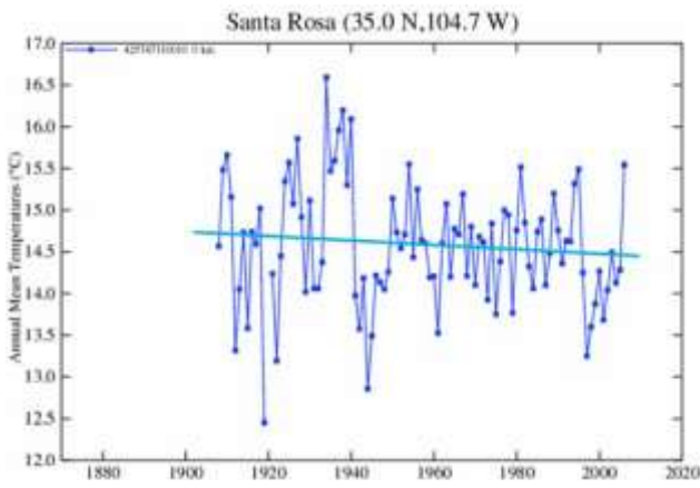
Figure 4.8: GISS Raw data showing cooling
