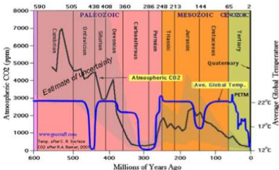
Figure 3.5: GEOCARB model of atmospheric CO 2 and temperature over the past 600 million years.
