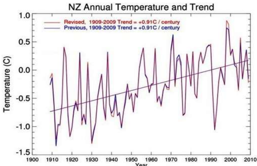
Figure 4.2: Adjusted NIWA temperature data (1910-2010) 50
