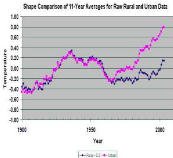
Figure 4.4: Raw USHCN Temperature Data (°F) 1900-2000
