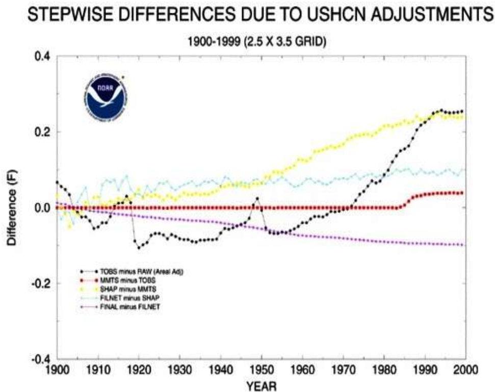
Figure 4.3: NOAA’s USHCN temperature data adjustments for 1900-2000.
