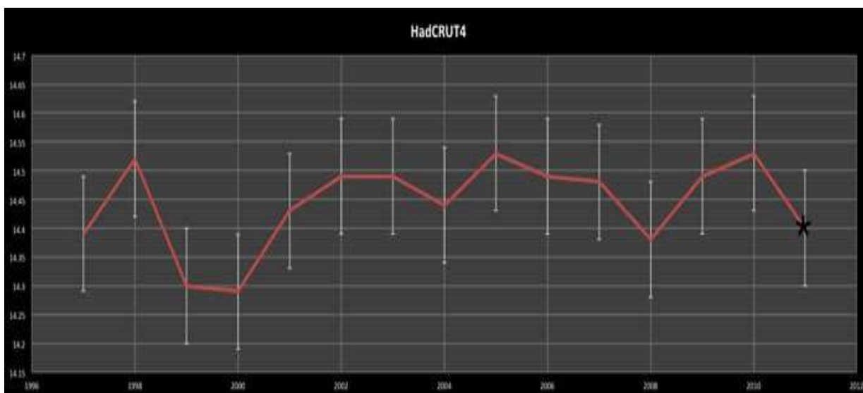
Figure 4.1: Annual mean surface temperature from 1997 to 2011. Source: Hadley Climate Research Unit
