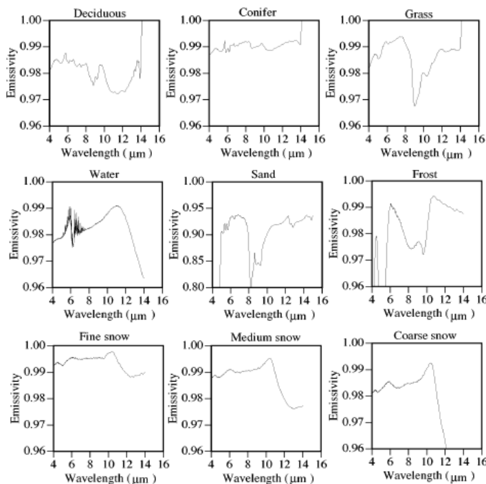
Figure 2.3: Emissivity from Laboratory Measurements for 9 Surfaces.
