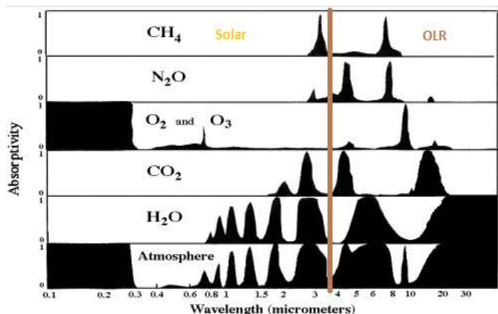
Figure 1.2: Absorption spectra of atmospheric gases individually and collectively (bottom). Solar IR is predominantly to the left of the red line and Earth’s OLR to the right of it. (1 micrometre \mu\text{m} = 1,000nm)
