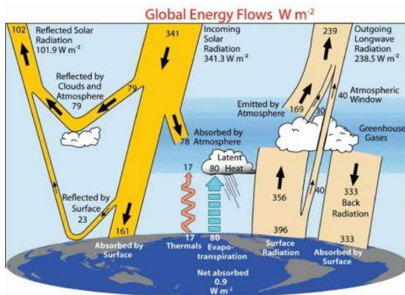
Figure 2.6: The global annual mean Earth's energy budget for the Mar 2000 to May 2004 (CERES) period (W m -2 ). The broad arrows indicate the schematic flow of energy in proportion to their importance. Source: Trenberth et al 2009
