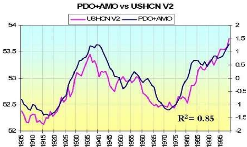
Figure 3.12: Pacific and Atlantic Oscillations vs. USA Temperature, 1905-2000.
