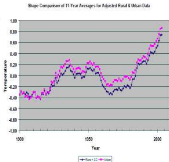
Figure 4.5: Adjusted USHCN Temperature Data (°F)
