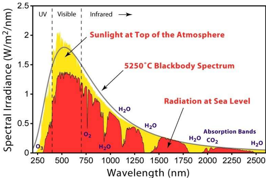
Figure 1.4: Solar Radiation Spectrum at Top of the Atmosphere (yellow) and at Sea Level (red).
