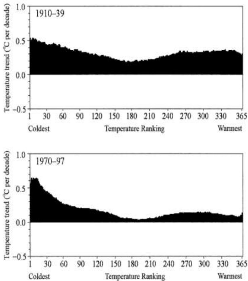
Figure 3.6: Trend in Night-time Low Temperatures (Day 1= coldest night, Day 2 = next coldest etc.) for 1910-39 (Top) and for 1970-97 (Bottom)
