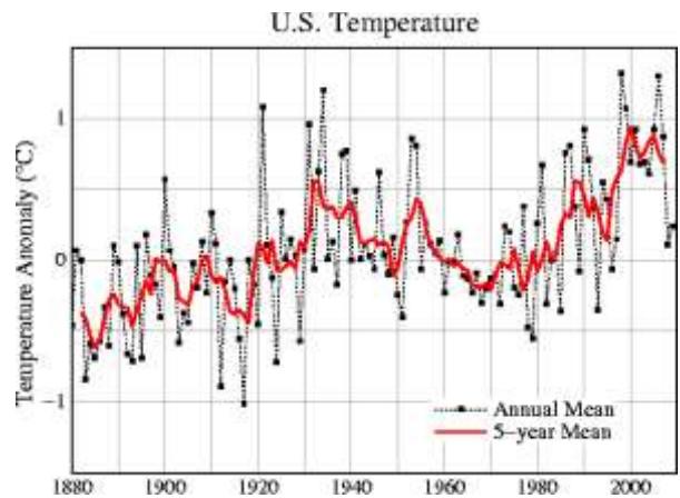
Figure 4.11: GISS 2010 processed US data
