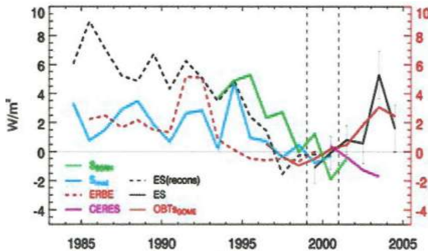
Figure 3.10: Annual albedo anomalies (relative to 1999-2001) derived from: Lunar Earthshine (ES) reconstructed (broken black) and actual (solid black); ERBE (broken red); OBT GOME (red); Satellite cloud S mod (blue) and S SBRN (green) Source: Palle et al, 2005 29
