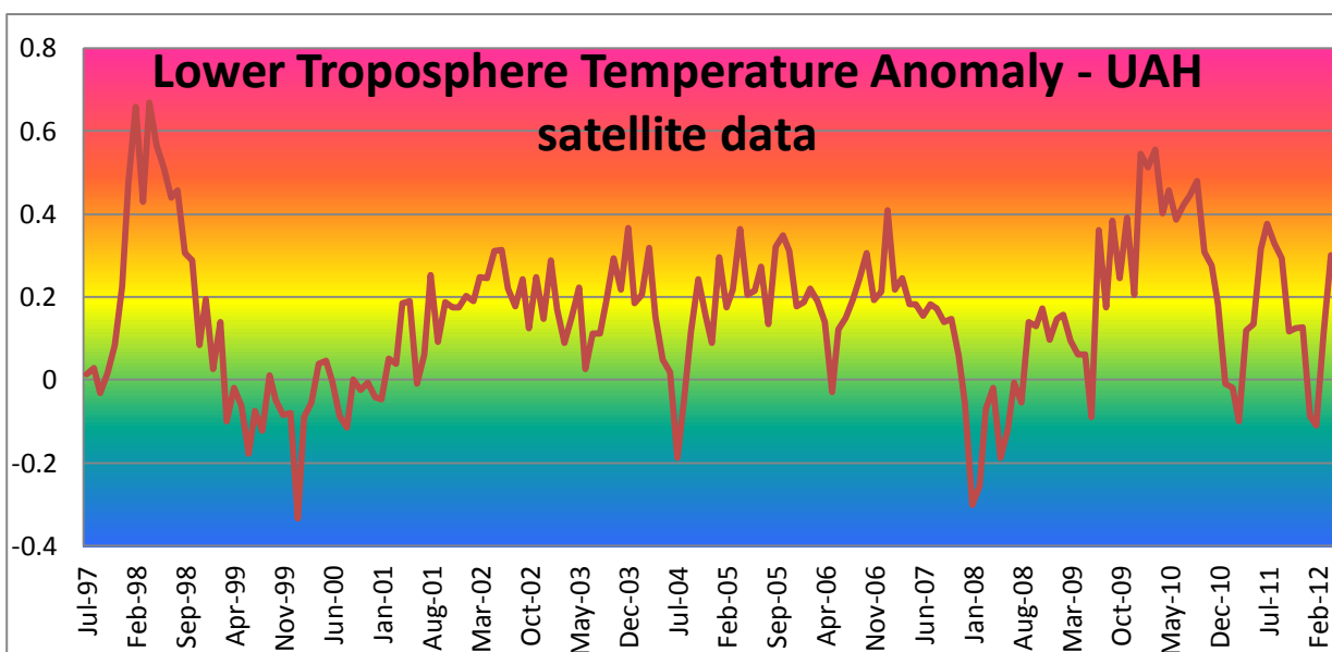
Figure 4.2: Monthly temperature anomaly of the lower troposphere over the last 15 years (1997 to 2012) Source: UAH satellite data (updated July 2012)
