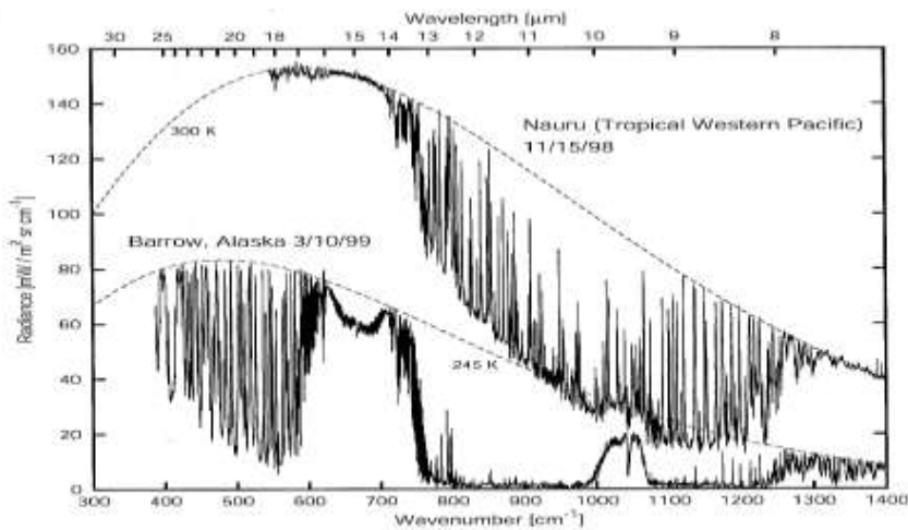
Fig. 8.1: Two examples of measured atmospheric emission spectra as seen from ground level looking up. Planck function curves corresponding to the approximate surface temperature in each case are superimposed (dashed lines). (Data courtesy of Robert Knuteson, Space Science and Engineering Center, University of Wisconsin-Madison.)
