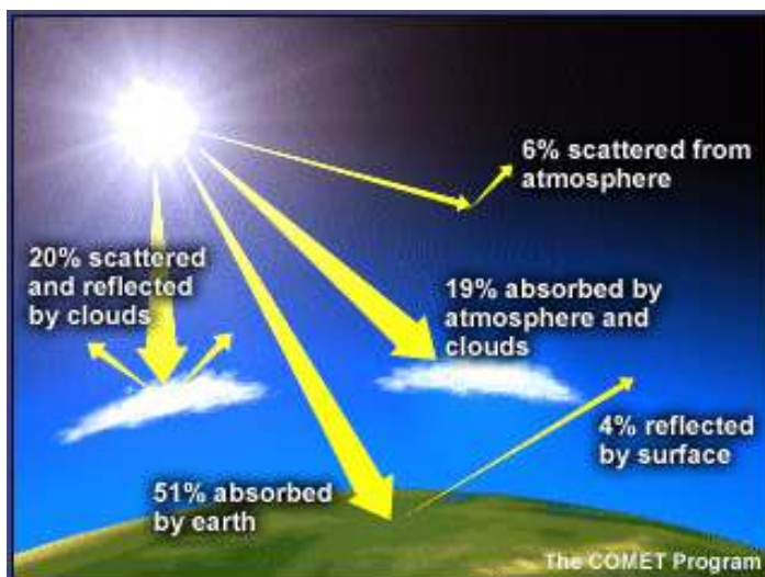
Figure 2.2: Interaction of Solar Radiation on Earth's Atmosphere and Surface
