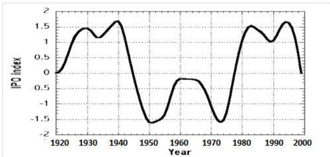
Figure 4.3: Interdecadal Pacific Oscillation (IPO) of Sea Surface Temperature (smoothed) 1920 to 2000. Source: Kiem et al, 2003
