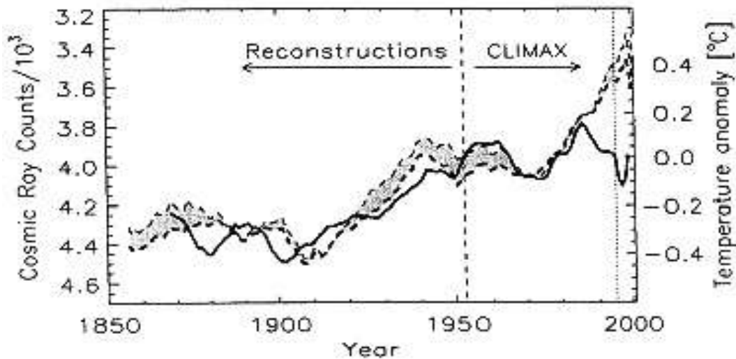
Figure 3.9: Cosmic ray flux (solid line) and global temperature anomaly from reconstructions pre-1952 and observations post-1952. Source: Krivova and Solanki, 2003
