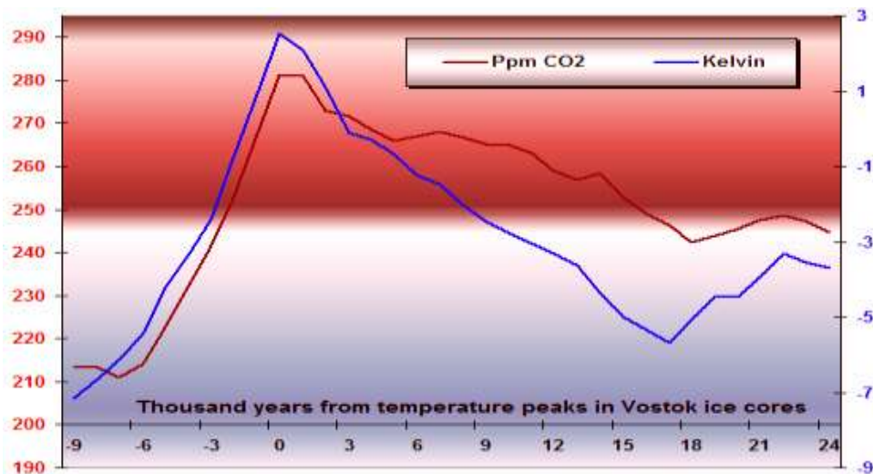
Figure 3.4: Compilation of actual data from all major temperature peaks in the Vostok Ice Core in Fig. 18
