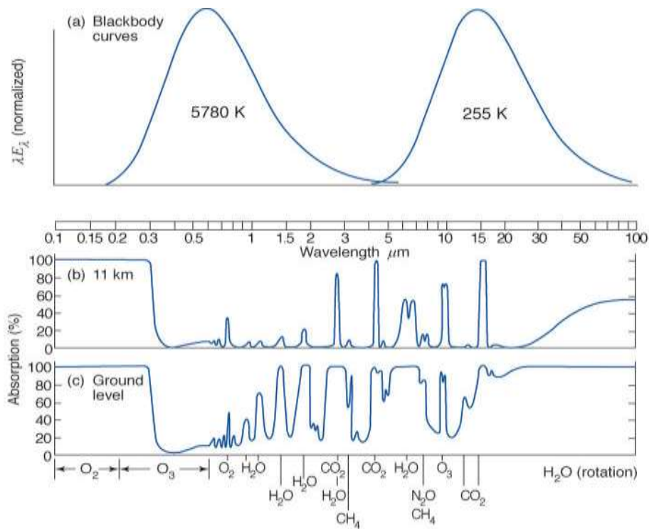
Figure 1.3: Top (a) – Blackbody spectral curves for the Sun (left) and Earth (right) Middle (b) – Absorption spectra at 11km altitude Bottom (c) – Absorption spectra for various greenhouse gases at ground level
