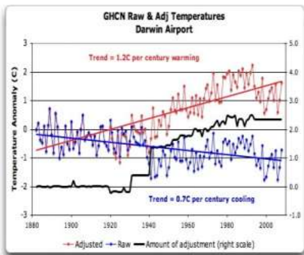
Figure 4.6: GHCN Adjustments to Darwin Airport
