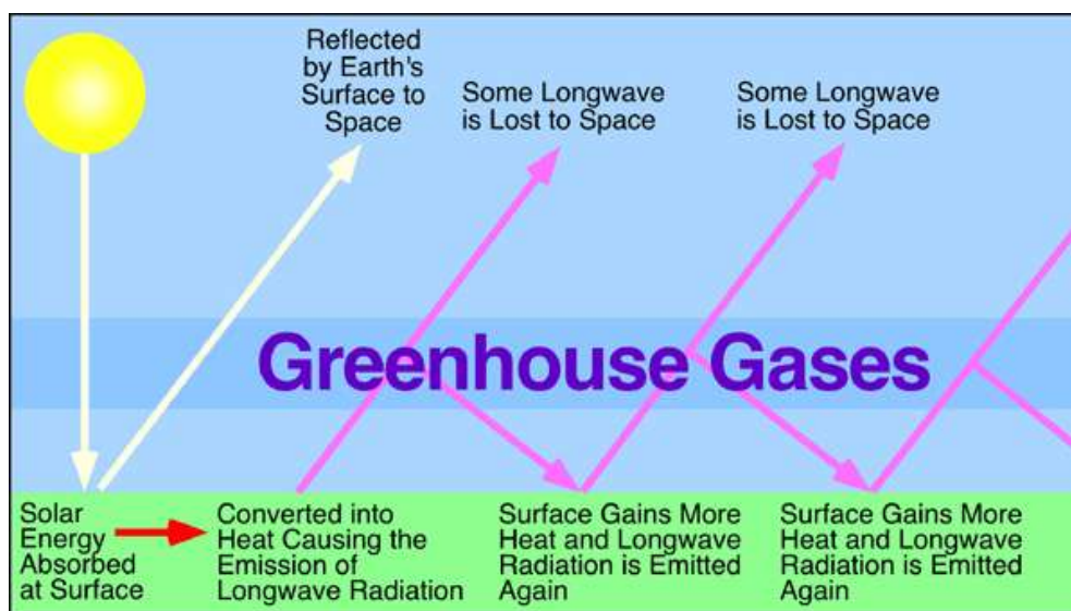
Figure 2.1: Greenhouse Theory according to Pidwirny .
