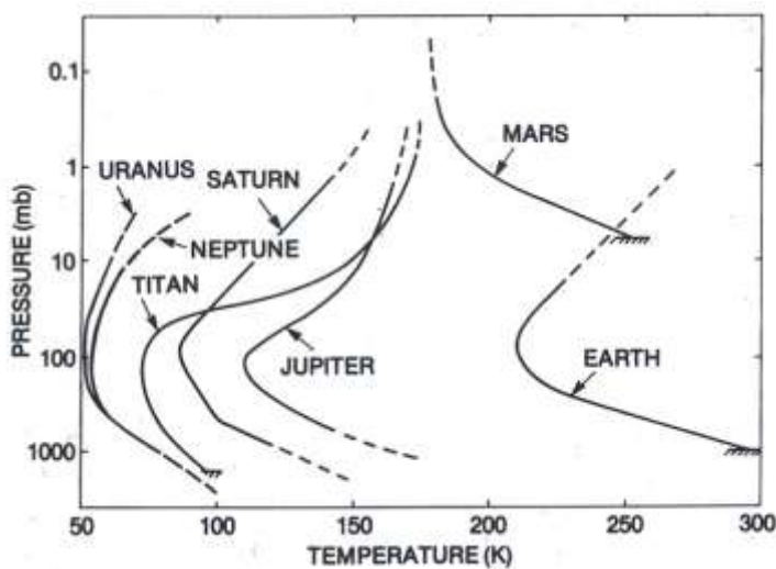
Figure 1.9 (8 in SSD): Pressure vs. Temperature of the Atmospheric Planets. Source: Colorado University
