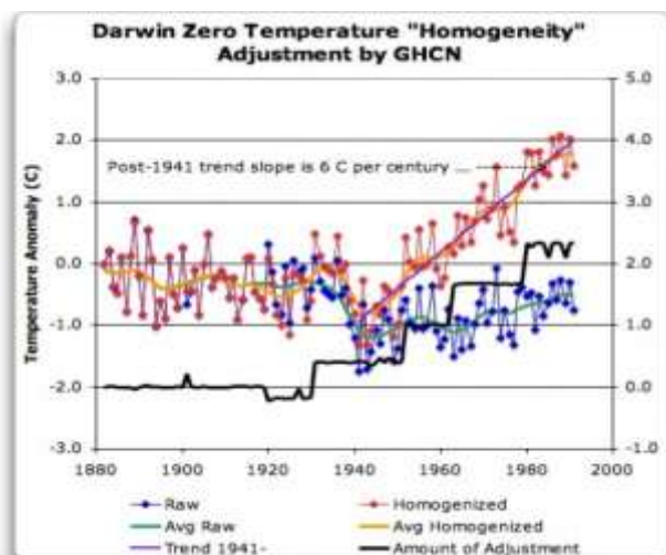
Figure 4.7: Homogeneity Adjustments at Darwin Zero.
