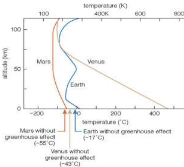
Figure 1.10: The postulated effect of atmospheric greenhouse gases on the surface temperature of Earth, Mars and Venus. Source: Colorado University
